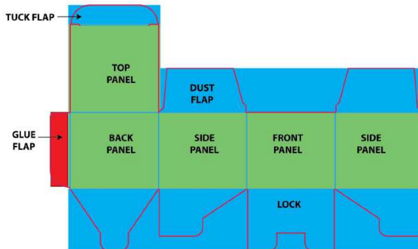
Lockbottom Box.
